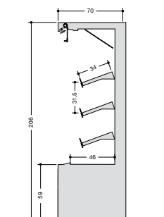
EI700-F
